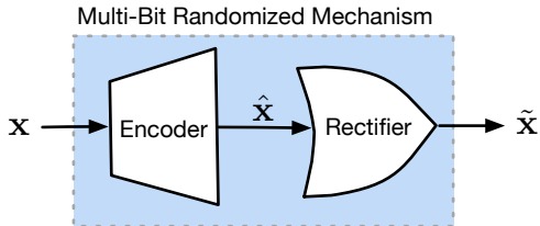
Fig. 3: Illustration of multi-bit mechanism. The encoder encodes the multi-dimensional features x_i \in \mathcal{R}^{|D|} into \hat{x}_i \in \{-1, 0, 1\}^{|D|} , with a probability defined by the privacy budget. The rectifier is to calibrate the encoded vector \hat{x}_i to ensure the outcome \tilde{x}_i is statistically unbiased.
