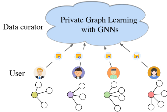
Fig. 1: The illustration of private learning over decentralized graph network: 1) each user holds a data share including a local neighbour list and the profile information; 2) the data curator collects the obfuscated data and conducts learning over the collected noisy graphs.
