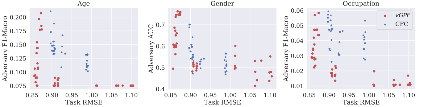
Fig. 7. Utility-Privacy trade-off plot for removing multiple attributes on MovieLens-1M. To compare with the compositional approach CFC, we train our variational model with compositional attributes s consisting of age, gender and occupation (by concatenation operator). We then use three adversarial classifiers instantiated with MLPs for inferring age, gender and occupation, respectively. Points located at the left bottom are better.
