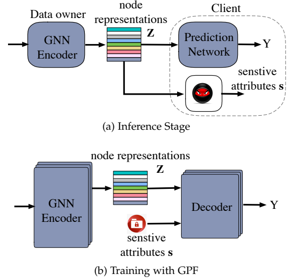
Fig. 1. (a) An illustration of the threat model in the inference stage. The client may want to infer sensitive attributes based on the representations received from the data owner. (b) An illustration of vGPF for training privacy-preserving GNN encoder at a trusted server. The decoder admits the representations from the GNN encoder and the sensitive attributes of interests. Once trained, the GNN encoder can extract graph representations that defend against attribute inference attacks in the inference stage.
